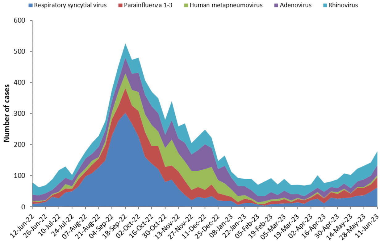
Figure 11. Number of non-influenza respiratory virus detections at PathWest by week, WA, 2022 to 2023 YTD
